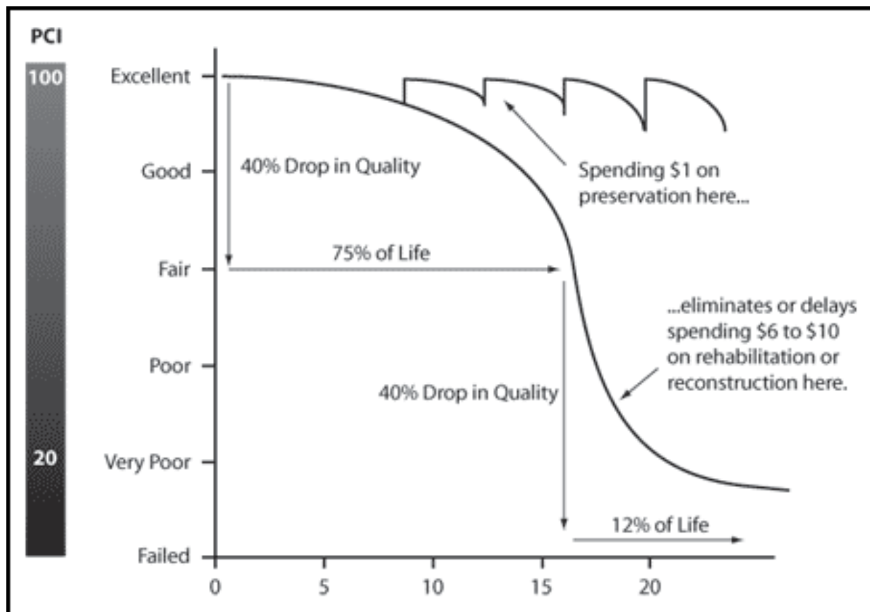
FIGURE 1: PAVEMENT DETERIORATION
